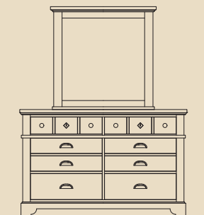
002 DRESSER 6-DRAWER 60 1/8 x 20 x 39 1/8 446 LANDSCAPE MIRROR 38 1/8 x 2 1/4 x 37 1/8
