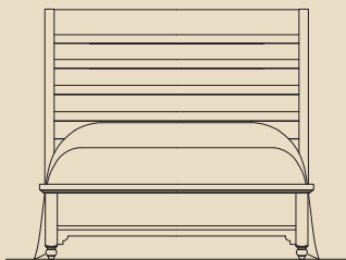
QUEEN 553 "ROGERS" SLEIGH HEADBOARD 63 1/4 x 12 1/2 x 60 1/2 955 LOW PROFILE FOOTBOARD 65 3/4 x 4 1/8 x 18 922 WOOD RAILS 82 x 1 x 5 3/4
