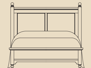
QUEEN 559 "GILCHRIST" POSTER HEADBOARD 63 x 2 7/8 x 58 955 LOW PROFILE FOOTBOARD 65 3/4 x 4 1/8 x 18 922 WOOD RAILS 82 x 1 x 5 3/4
