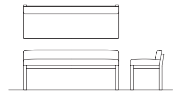
Upholstered Bench Bench: 080 50 3/4 x 20 x 24 1/4
